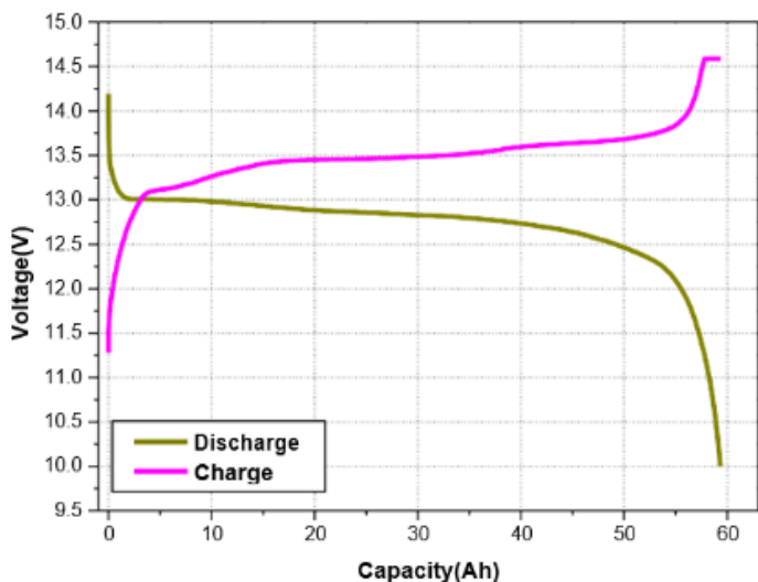
12.8 V – 121.6 Ah Charge-Discharge Curve 0.2 C, 25 °C
