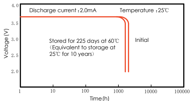
3. Storage characteristics
